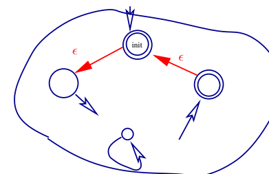
Automaton for L^*
