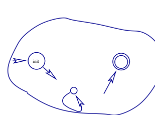
Automaton for L
